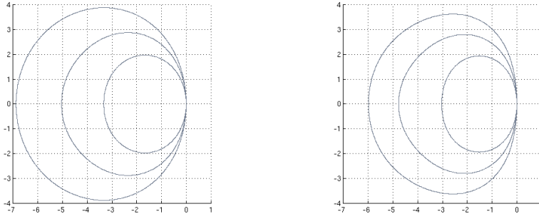
Figure 2: Stability regions of optimally smoothing methods for CFL = 3 (left) and CFL = 24 (right). The larger the stability region, the higher the number of stages.
