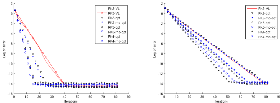
Figure 8: Convergence plots for different methods for step function initial data with nonperiodic boundary conditions: CFL 3 (left) and CFL 24 (right).
