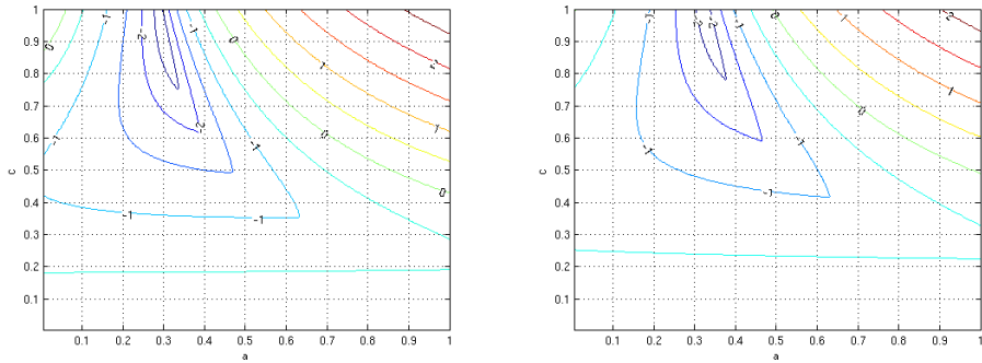
Figure 1: Contourplots of functions \log_{10} \max_{|\Theta| \in [\pi/2, \pi]} |P_2(z(\Theta, c; 3))|^2 (left) and \log_{10} \max_{|\Theta| \in [\pi/2, \pi]} |P_2(z(\Theta, c; 24))|^2 (right).
