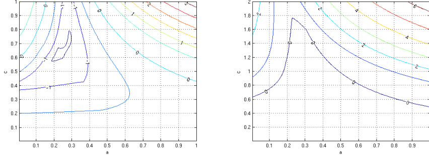
Figure 3: 2-stage method: Contourplots of \log(\rho(\mathbf{M}(\alpha, c))) for \Delta x = 1/24 and \nu = 0.125 (left) and \nu = 1.0 (right).
