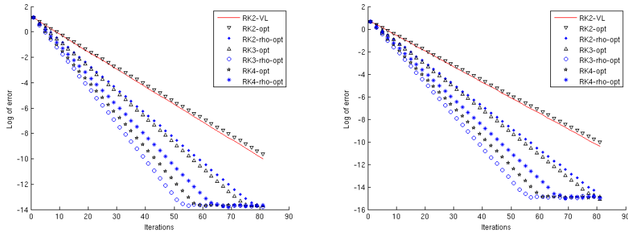
Figure 7: Convergence plots for different methods and CFL = 24 : step function (left) and sine initial data (right).
