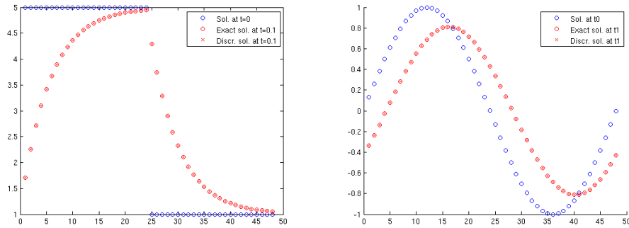
Figure 5: Initial solution and discrete and numerical solution after one time step for step function (left) and sine initial data (right).
