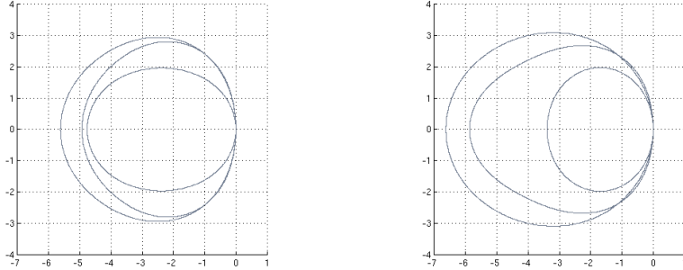
Figure 4: Stability region of optimal 2-, 3- and 4-stage method for \Delta x = 1/24 and \nu = 0.125 (left) and \nu = 1.0 (right). The larger the number of stages, the larger the stability region.
