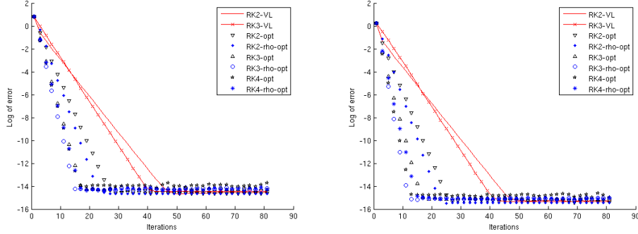
Figure 6: Convergence plots for different methods and CFL = 3 : step function (left) and sine initial data (right).
